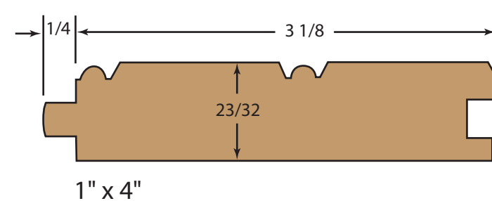
1" x 4"
