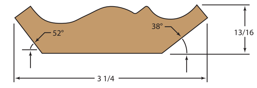
3 1/4" Crown
