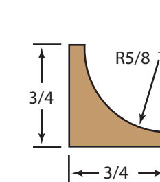
Cove Mould
