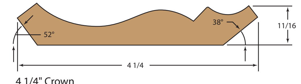
4 1/4" Crown
